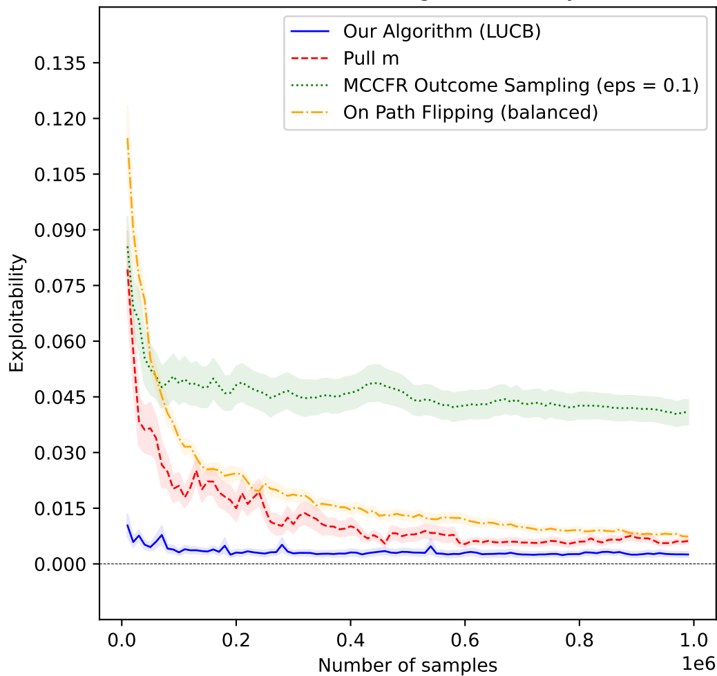
Leduc Poker, Best Algorithm, Player x
